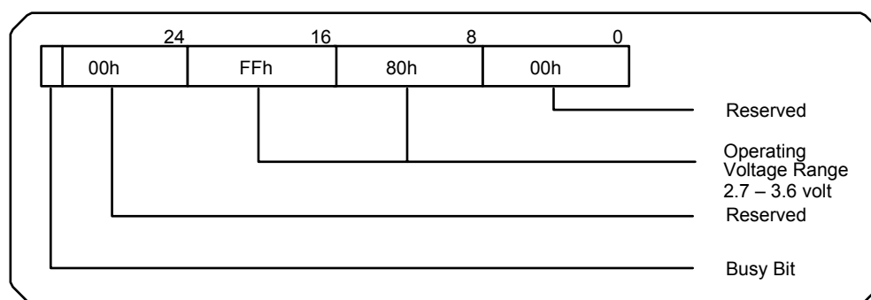
Figure 4-6 OCR Structure
