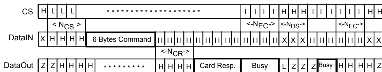
Figure 6-14 Timing Diagram of Command/Response Transaction, Card is Busy
