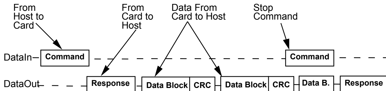
Figure 6-3 Multiple Block Read Operation
