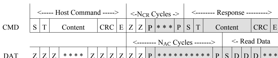
Figure 5-10 Transfer of Single Block Read
