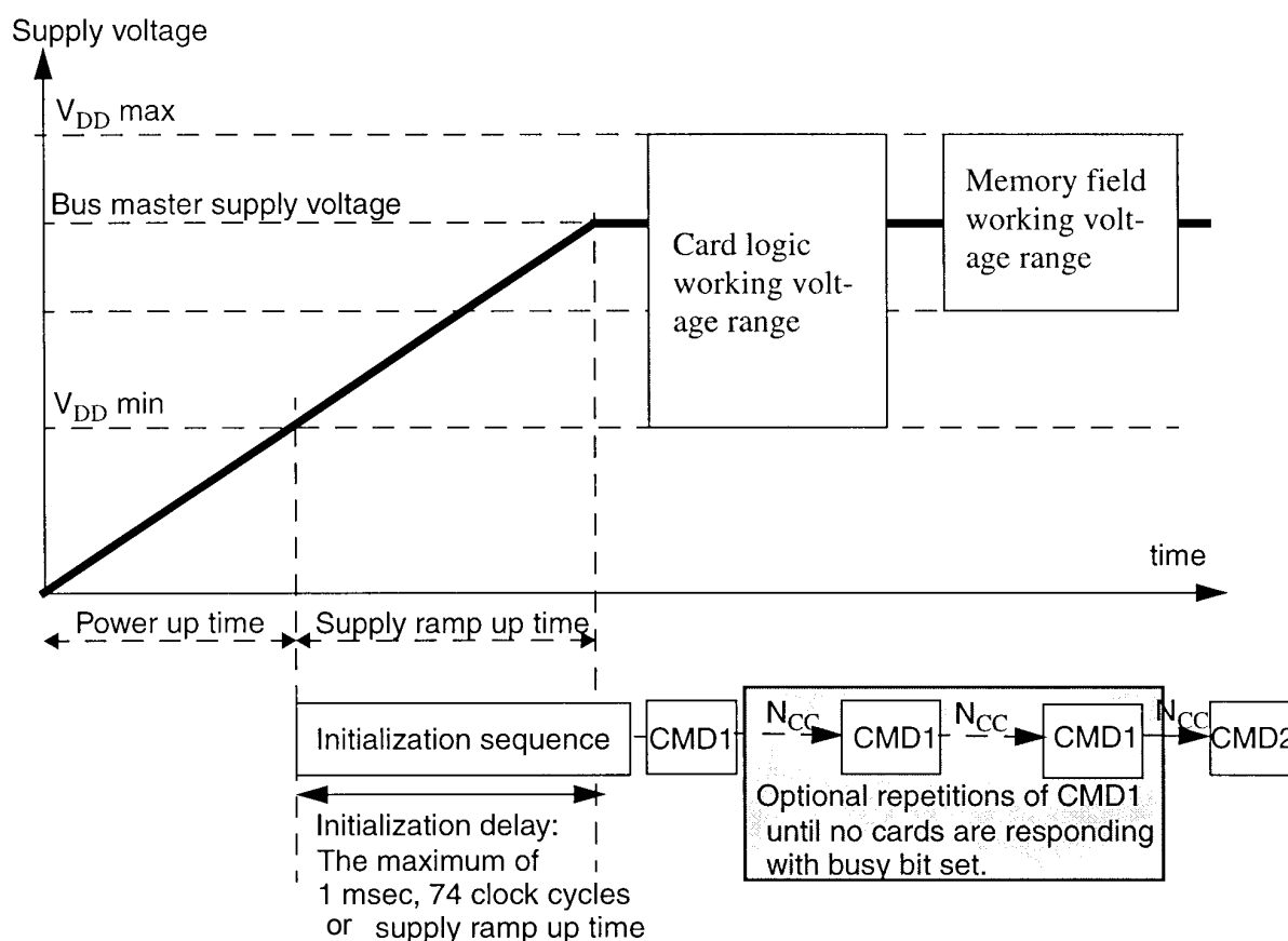
Figure 4-3 Power-up Diagram
