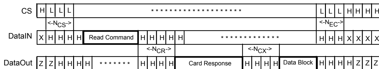
Figure 6-19 Timing diagram: Read CSD Register
