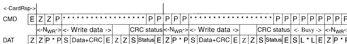
Figure 5-14 Timing of Multiple Block Write Command
