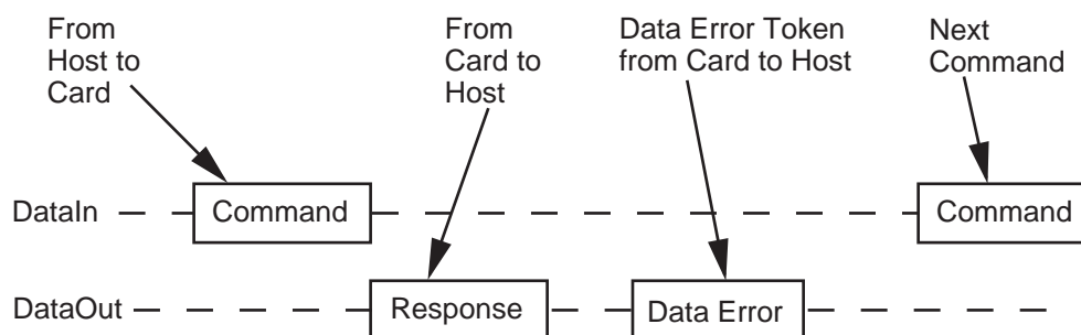
Figure 6-4 Read Operation - Data Error
